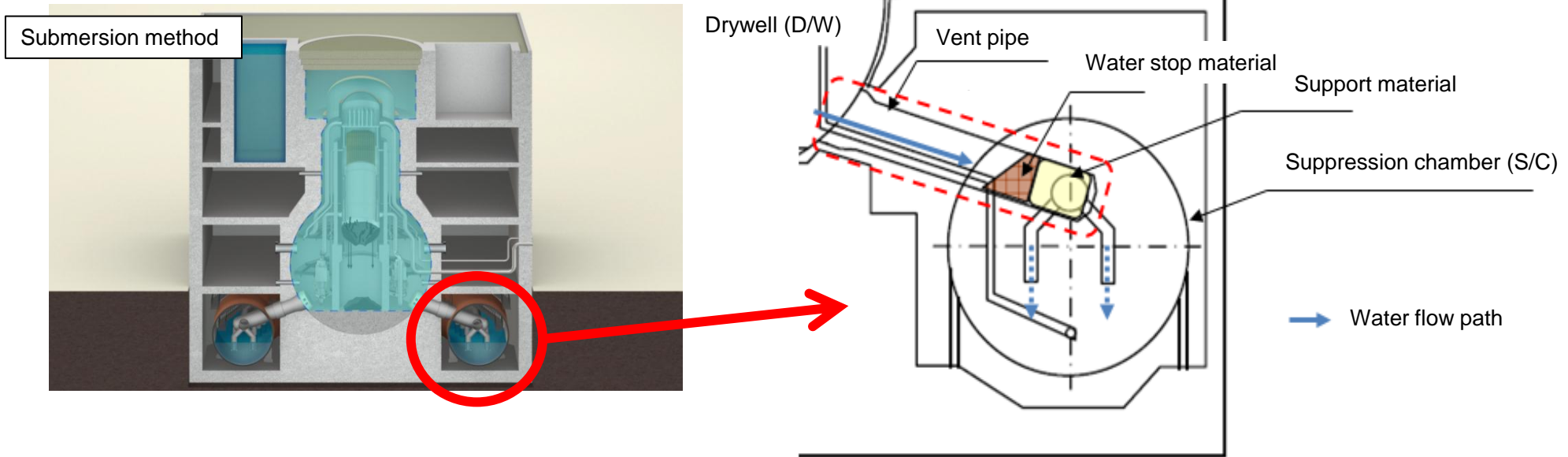
Area subject to repair in the lower section of the PCV
